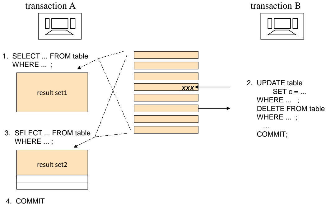
Figure 2.4 Non-repeatable Read problem in transaction A
